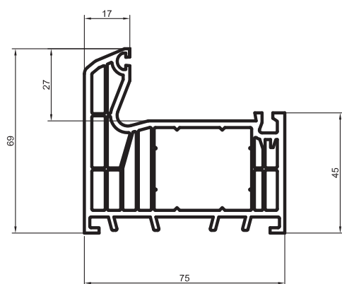
Ablak tok penta plus 2514
