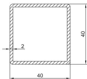
Merevítő 3533 Fe/Zn I_x = 7,21\text{cm}^4 I_y = 7,21\text{cm}^4
