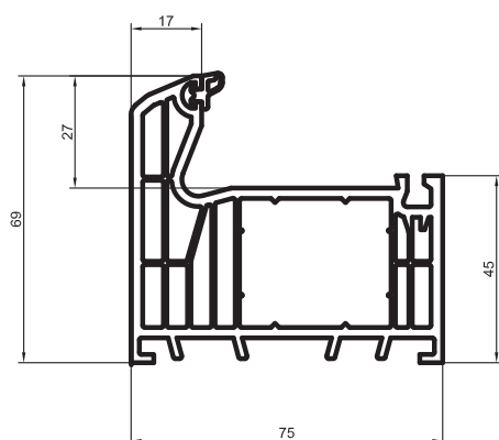
Ablak tok penta plus 2515
